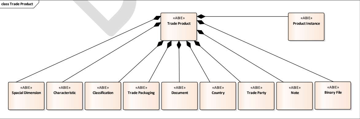
Figure 7-9 Business Entity Class Diagram – Trade Product
