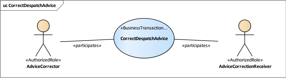
Figure 7-4 Business Transaction Use Case Diagram Correct Despatch Advise
