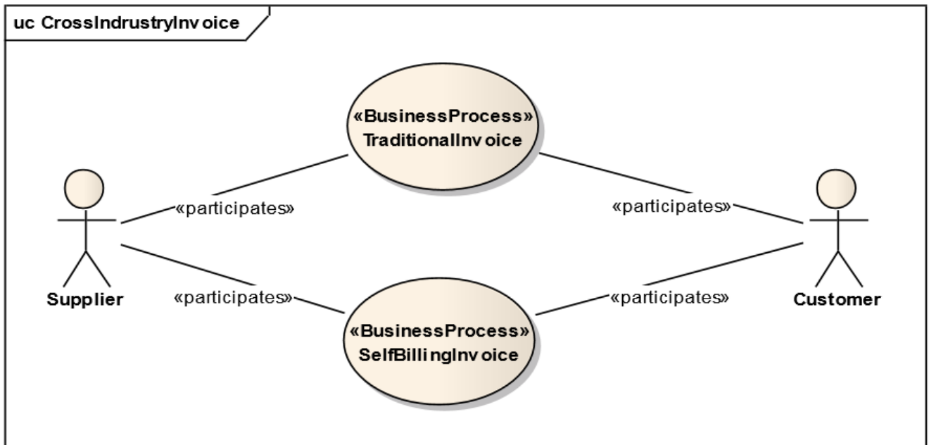
Figure 5-13 Business Process Use Case Diagram
