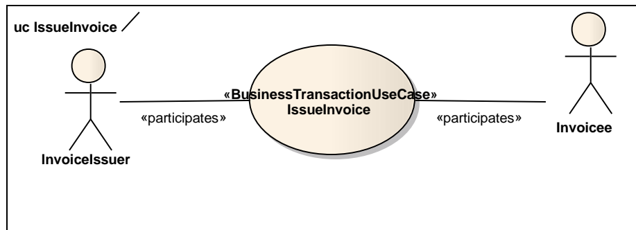
Figure 5-17 Business Transaction Use Case Diagram
