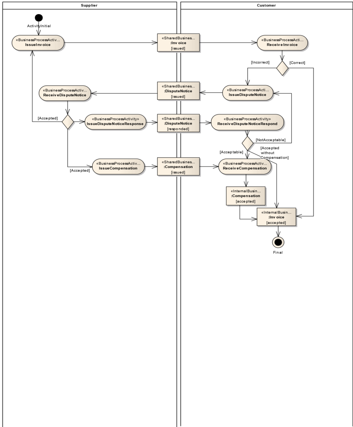
Figure 5-2 Business Process Activity Diagram
