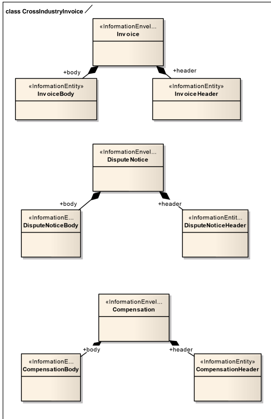
Figure 5-21 Business Entity Class Diagram
