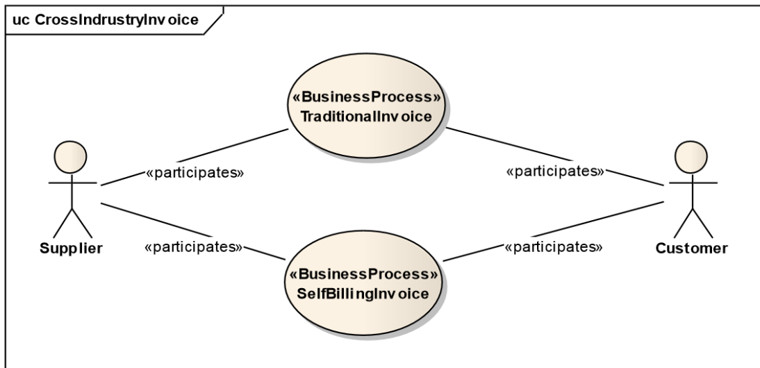
Figure 5-9 Business Process Use Case Diagram
