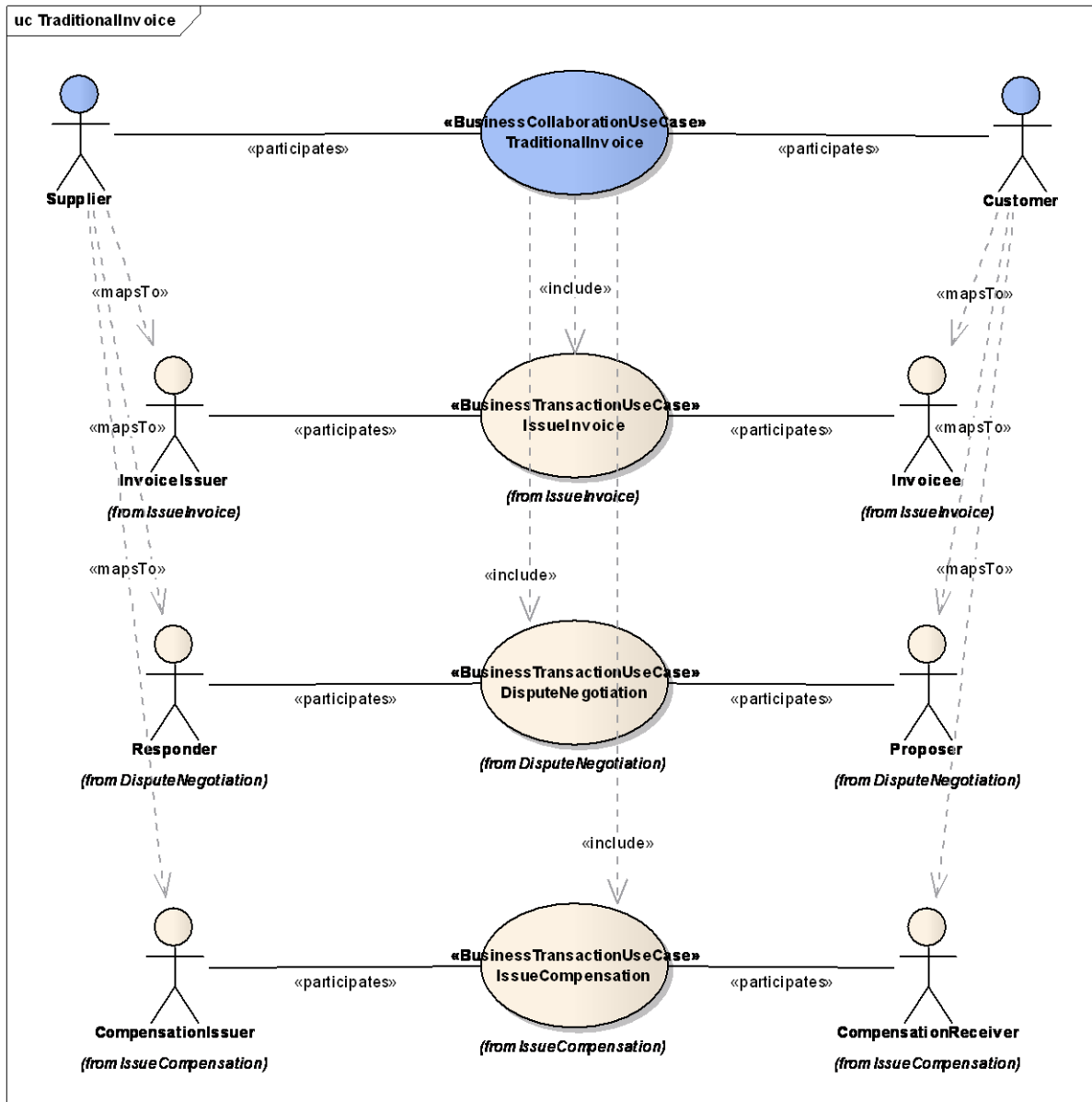
Figure 5-3 Business Collaboration Use Case Diagram
