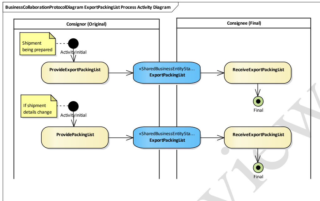
Figure 8-2 Business Process Activity Diagram
