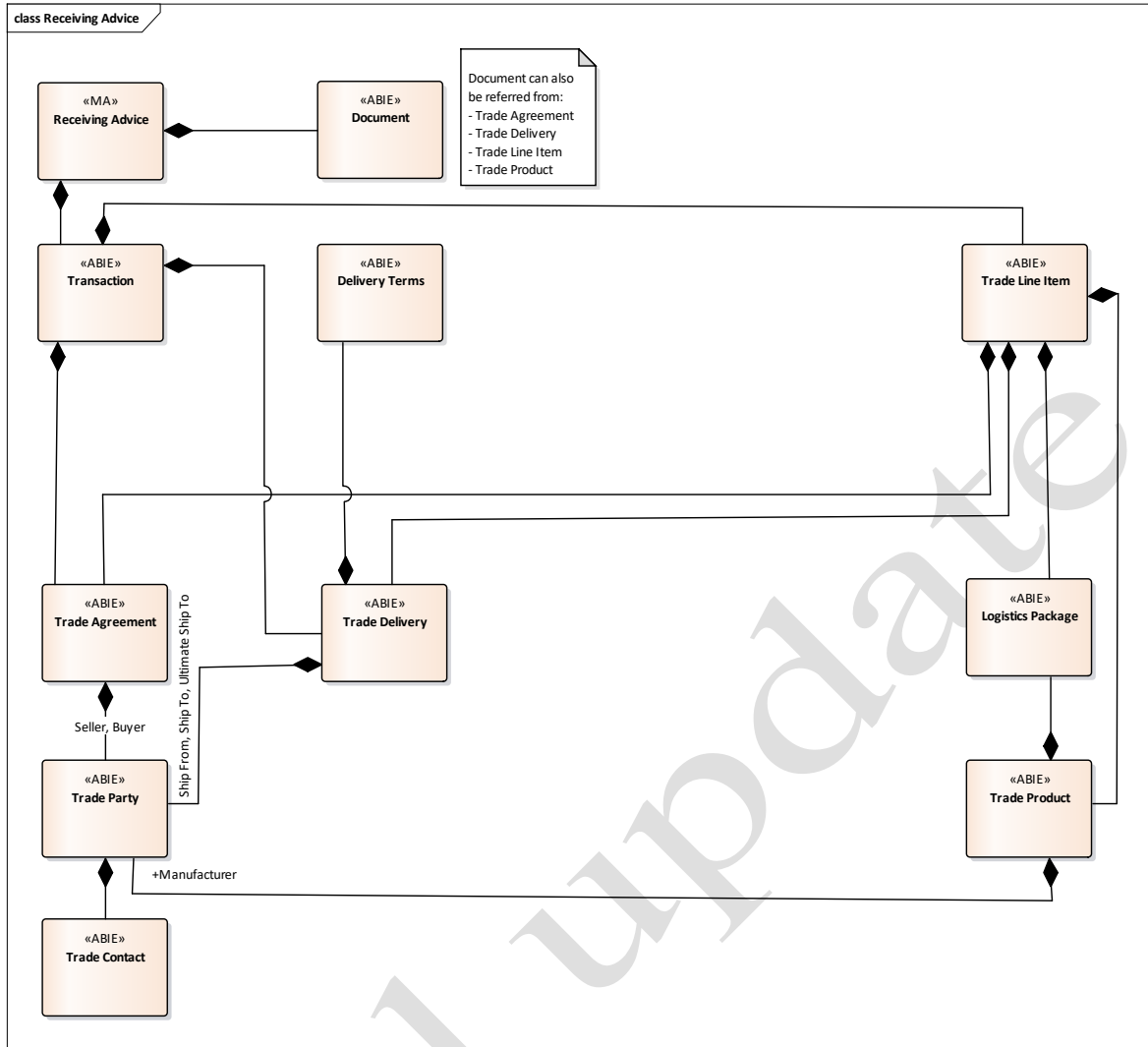
Figure 8-9 Business Entity Class Diagram – Receiving Advice
