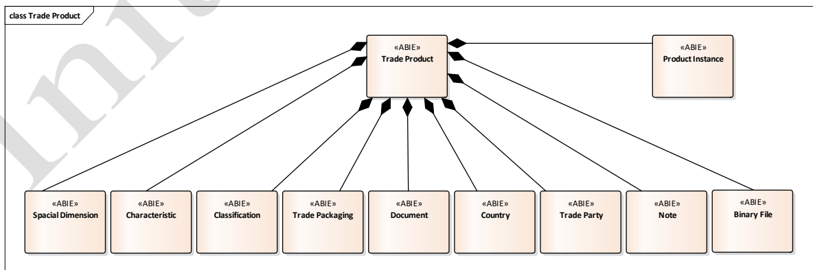
Figure 8-10 Business Entity Class Diagram – Trade Product
