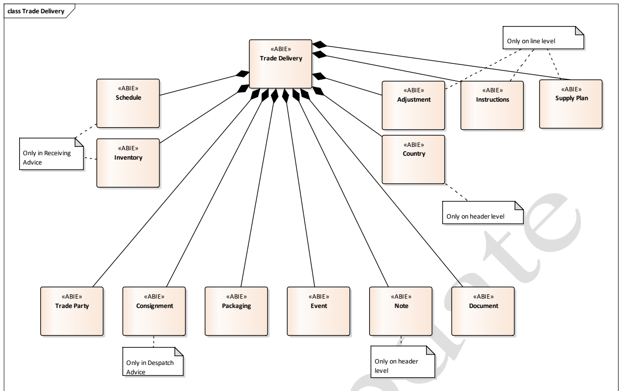
Figure 8-11 Business Entity Class Diagram – Trade Delivery
