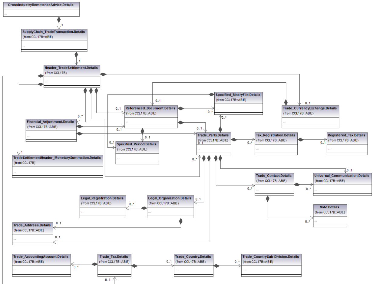
Figure 4 Header Trade Settlement
