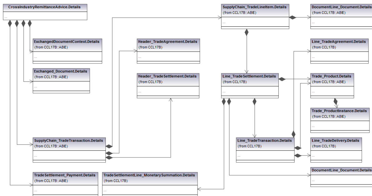
Figure 1 Cross Industry Remittance Advice conceptual data model
