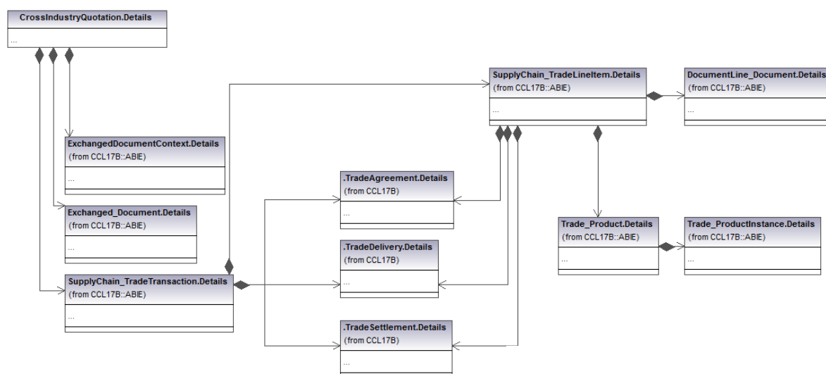
Figure 1 Cross Industry Quotation conceptual data model
