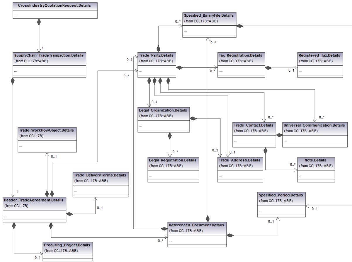
Figure 3 Header Trade Agreement
