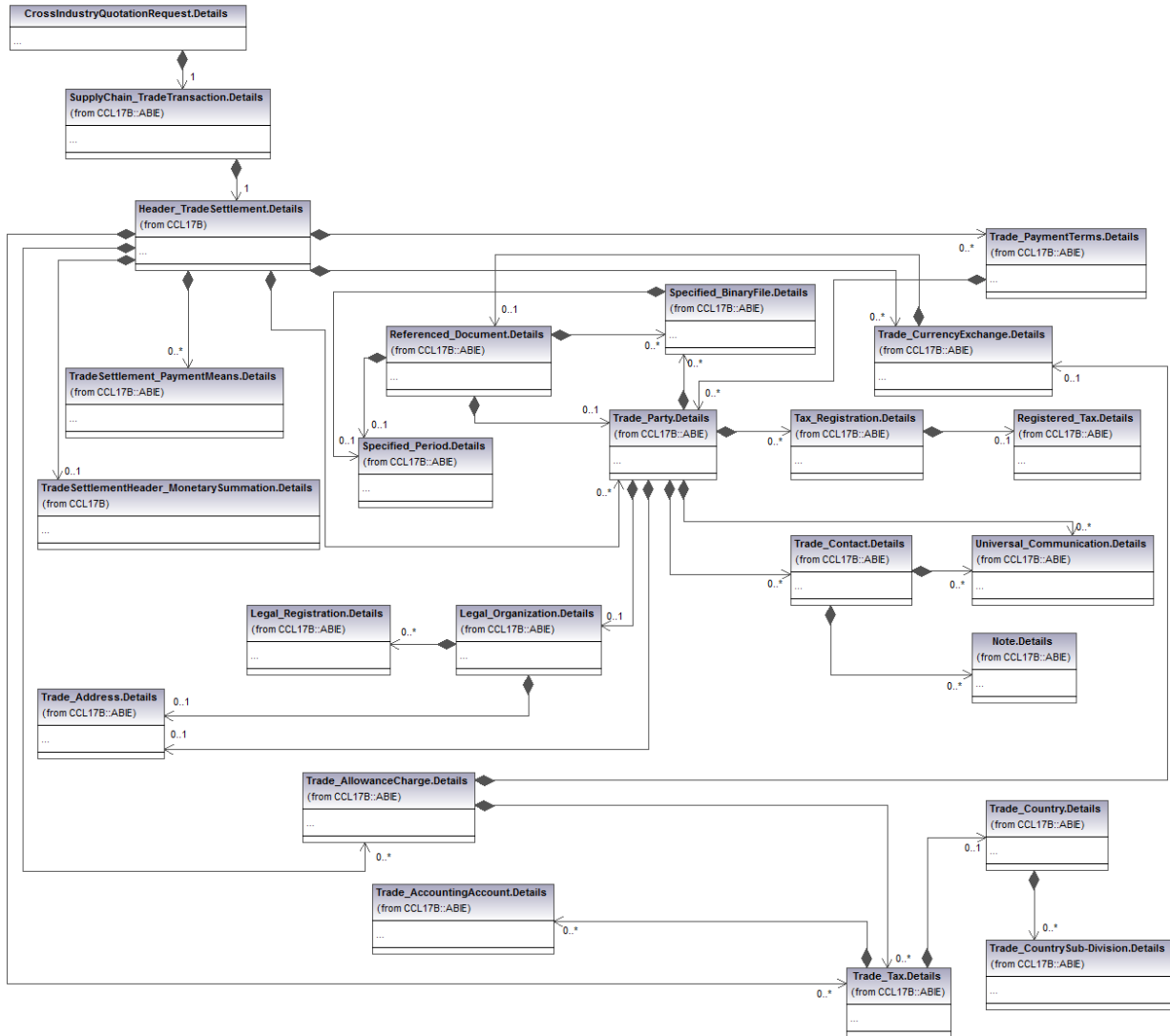
Figure 5 Header Trade Settlement
