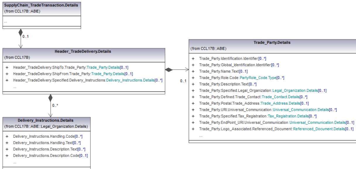
Figure 13 Header Trade Delivery
