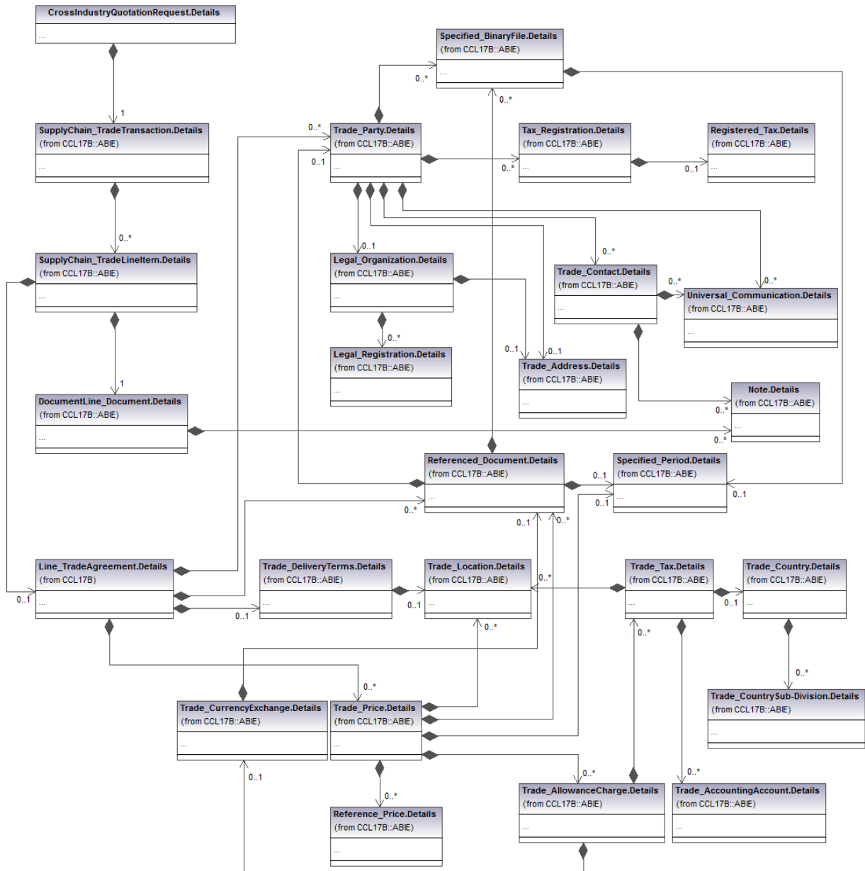
Figure 6 Line Trade Agreement
