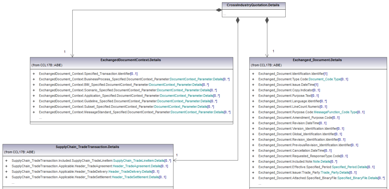
Figure 10 Cross Industry Quotation (root elements)
