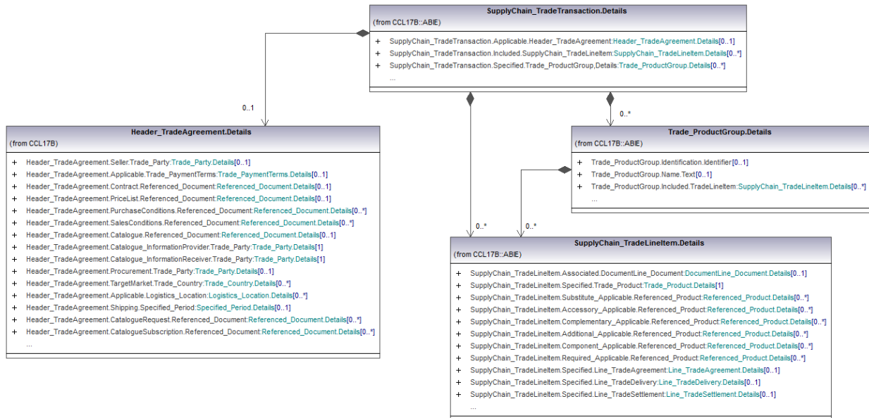
Figure 9 Trade Transaction
