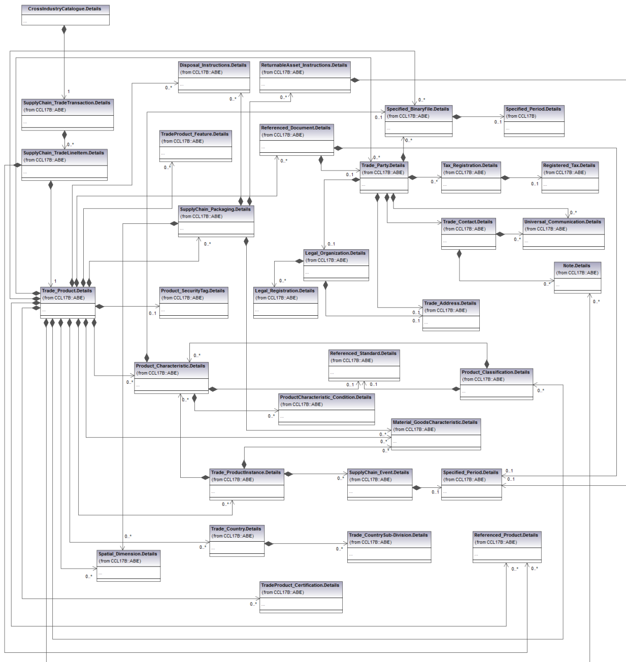
Figure 7 Trade Product
